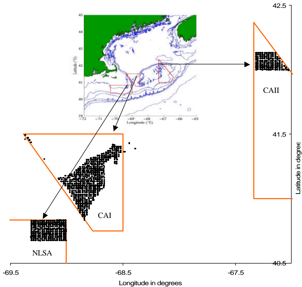
Figure 26. CMAST video survey conducted in Nantucket Lightship Area (NLSA), Closed Area I (CAI) and Closed Area II (CAII) during the May to September 1999.
